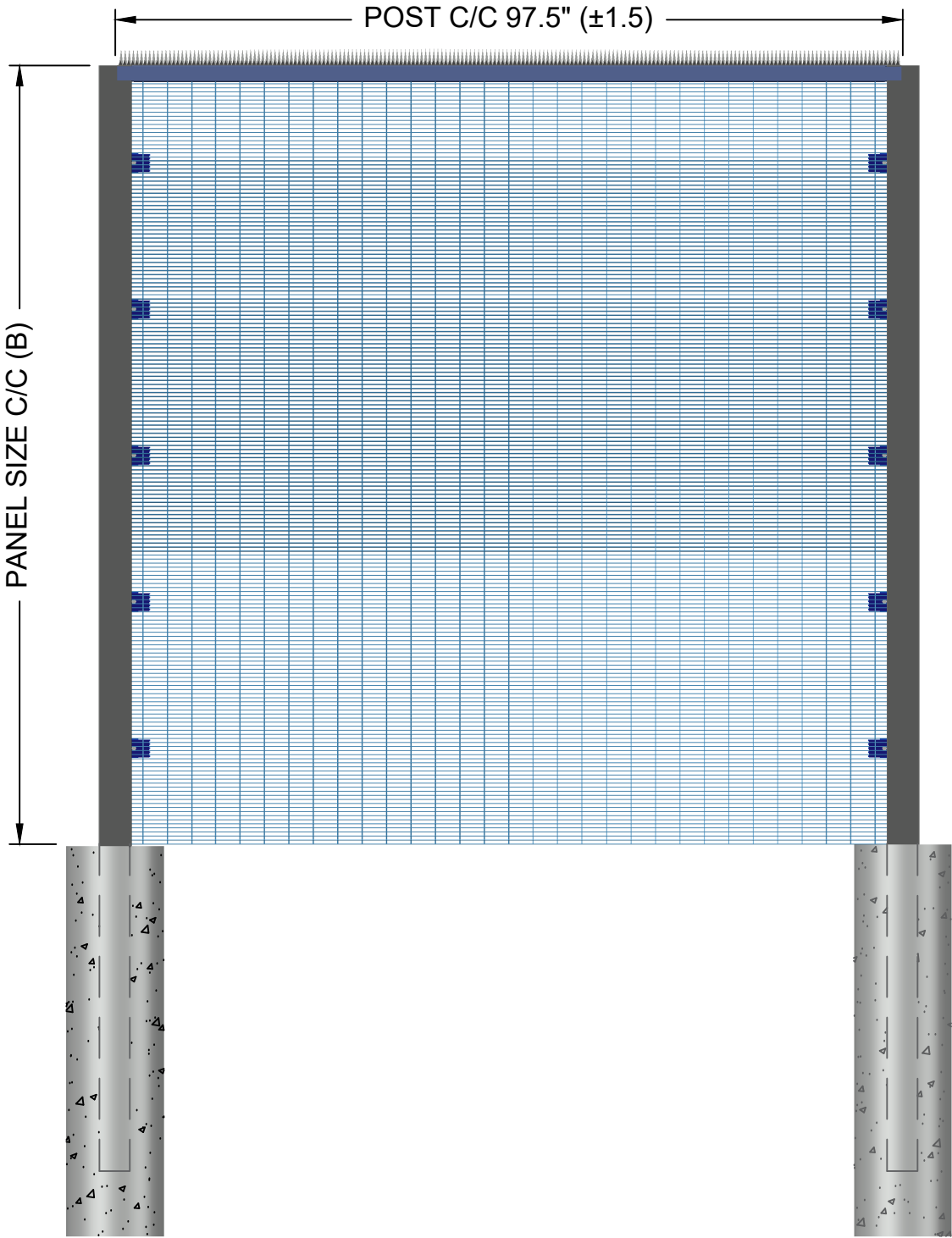
ELEVATION VIEW
