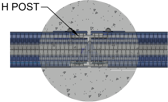
PANEL FIXING DETAIL
