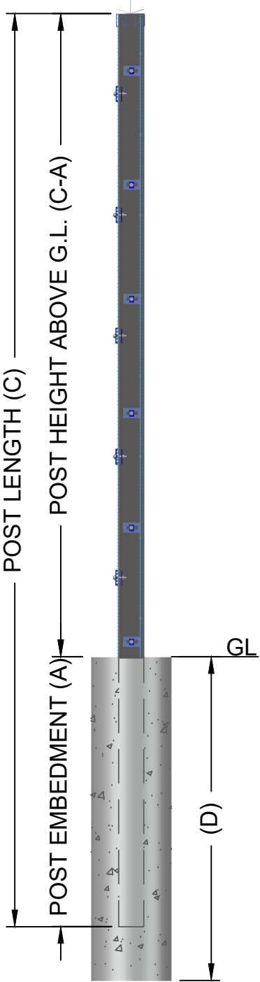
SIDE VIEW
