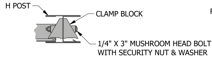
F - DETAIL AT POST
