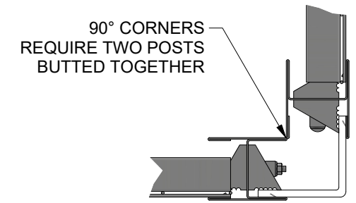
90° OUTSIDE CORNER DETAIL AT POST
