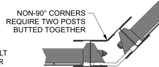
NON-90° CORNER DETAIL AT POST
