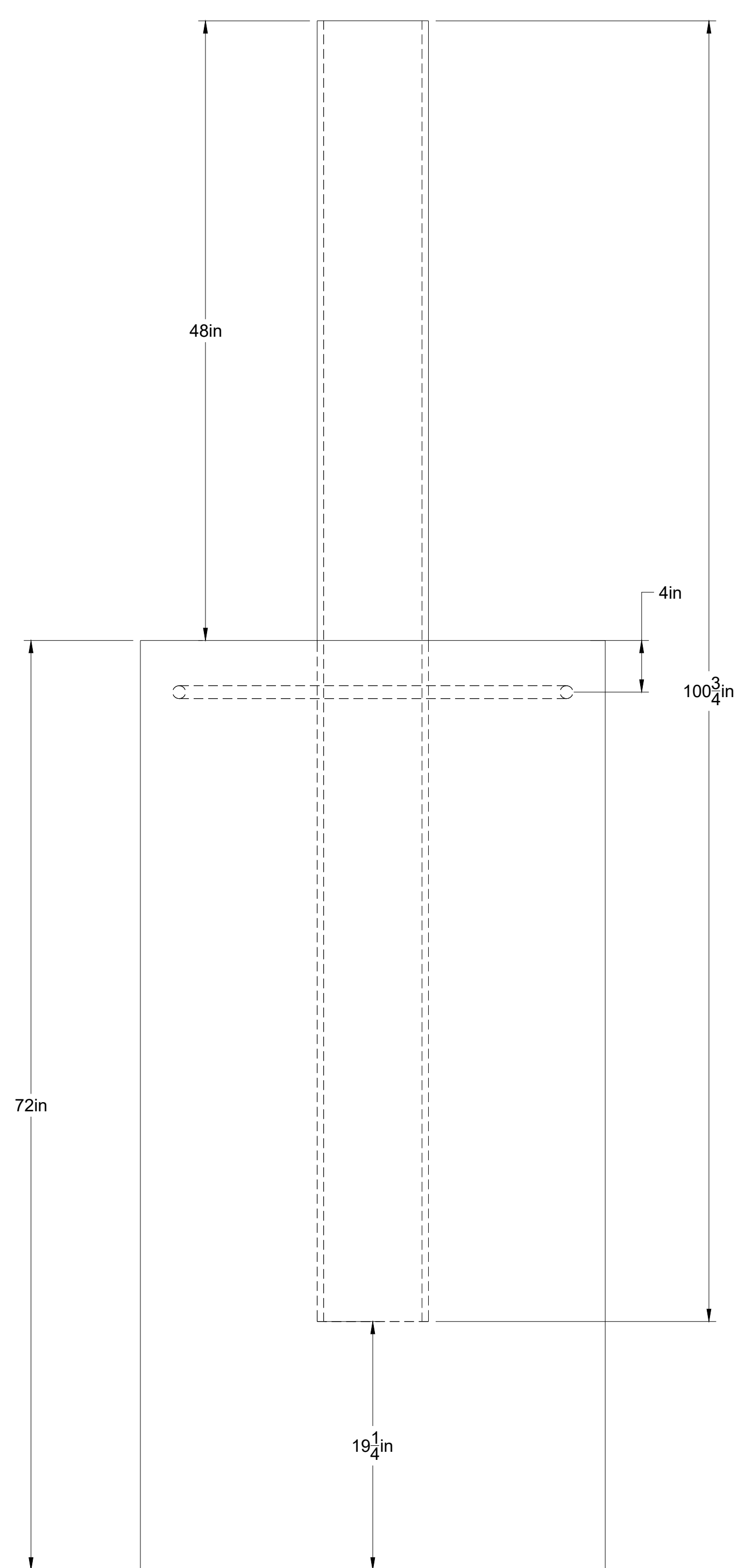
Elevation View
