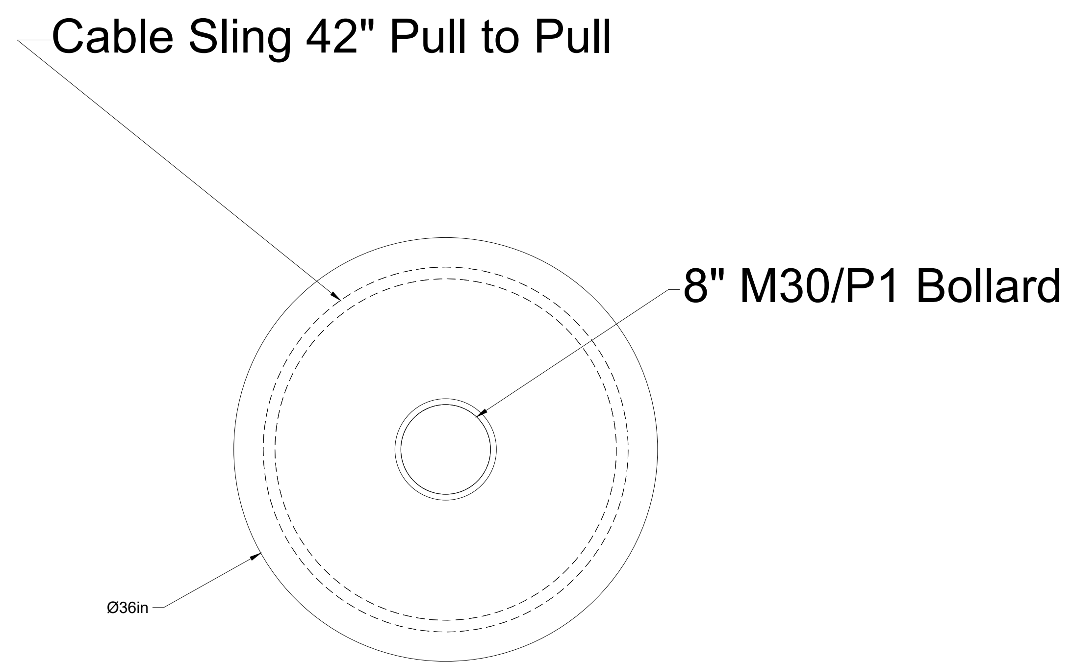
Plan View
